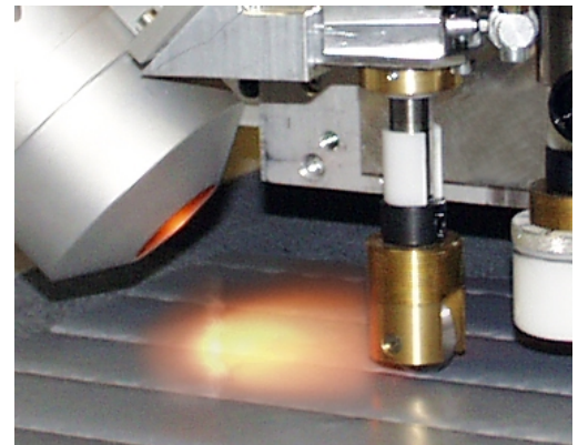
Permanent deformation by well-aimed cone of light.
